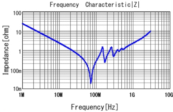
■ GCM55Q7U3A682JX01 |Z| DC0V, 25degC
