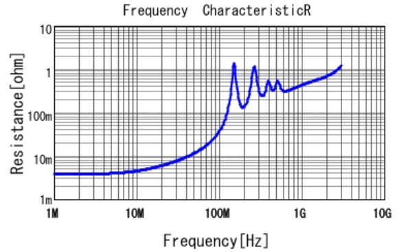
■ GCM55Q7U3A682JX01 R DC0V, 25degC
