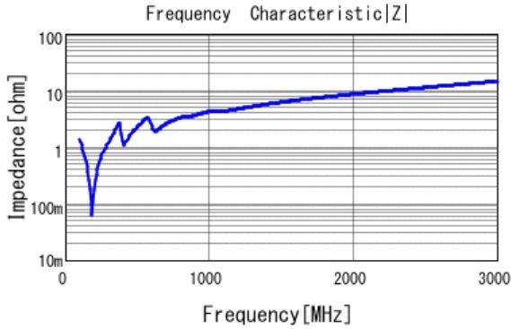
■ GCM31C5C3A821JX03 |Z| DC0V, 25degC
