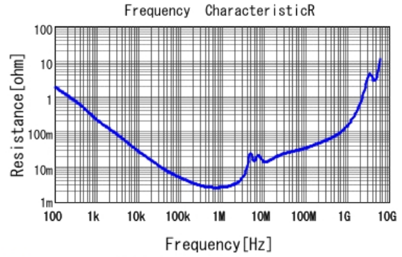
■ GCM32ER71H475KA55 R DC0V, 25degC
