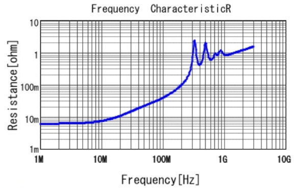
■ GCM31C7U3A102JX03 R DCOV, 25degC
