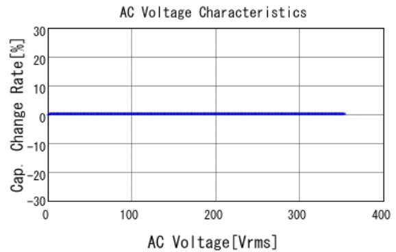
■ GCM31C7U3A102JX03 C-AC Voltage capchange, DCOV, 25.0d
