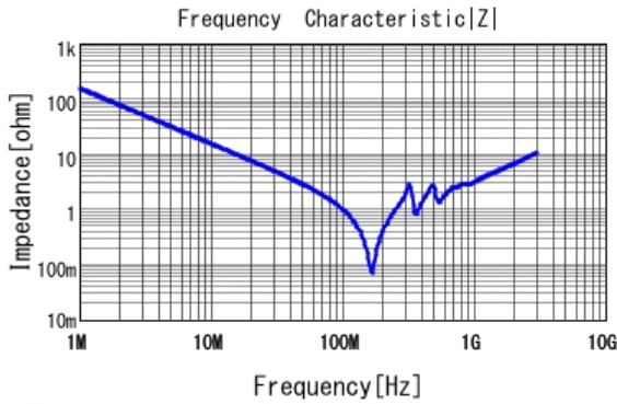
■ GCM31C7U3A102JX03 |Z| DCOV, 25degC
