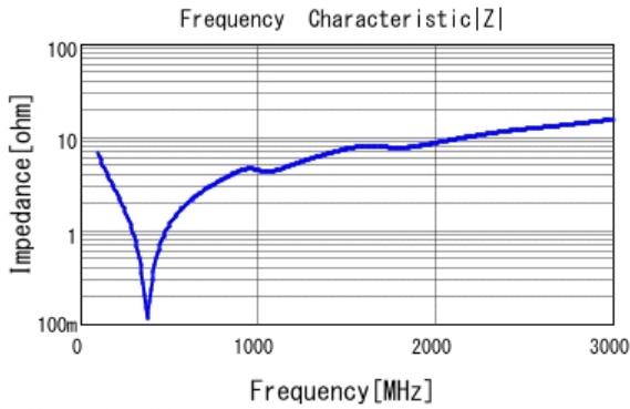
■ GCM31A7U3A221JX01 |Z| DC0V, 25degC
