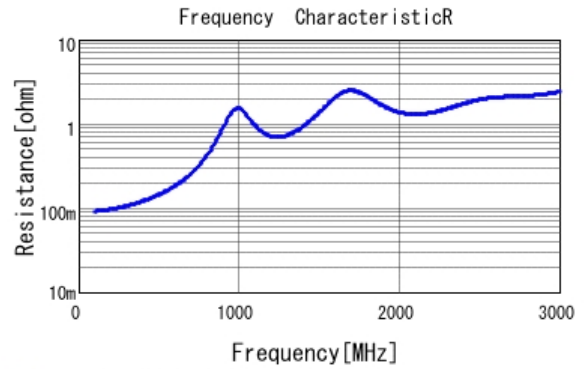
■ GCM31A7U3A221JX01 R DC0V, 25degC
