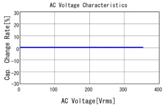
■ GCM31A7U3A221JX01 C-AC Voltage capchange, DC0V, 25.0d
