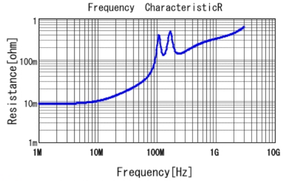
GCM31B7U2E103JX01 R DC0V, 25degC
