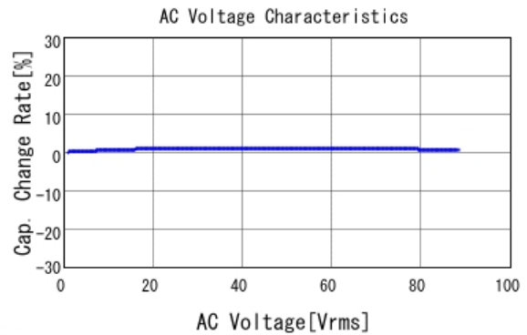
GCM31B7U2E103JX01 C-AC Voltage capchange, DC0V, 25.0d
