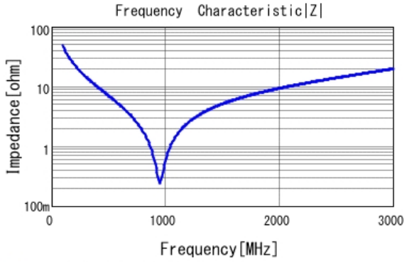
■ GCM31A7U2J330JX01 |Z| DC0V, 25degC
