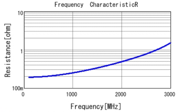
■ GCM31A7U2J330JX01 R DC0V, 25degC
