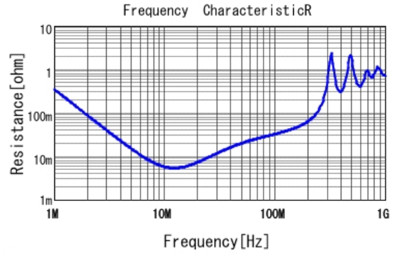
GCM31C5C3A102JX03 R DC0V, 25degC
