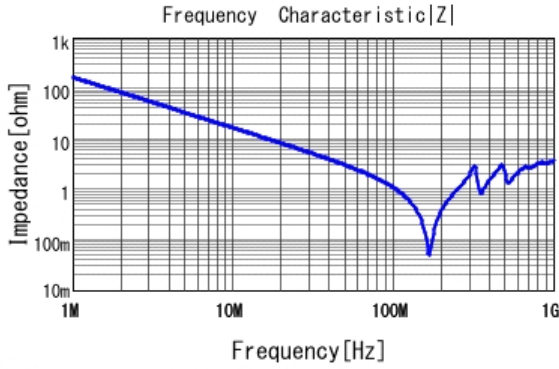
GCM31C5C3A102JX03 |Z| DC0V, 25degC
