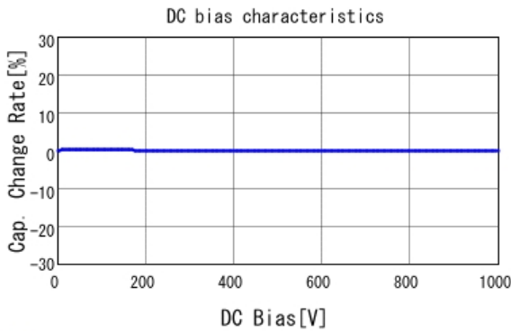
GCM31C5C3A102JX03 C-DC bias capchange, 25.0degC, AC1V
