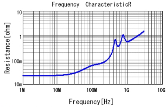
■ GCM31A7U2J102JX01 R DCOV, 25degC
