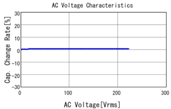
■ GCM31A7U2J102JX01 C-AC Voltage capchange, DCOV, 25.0d
