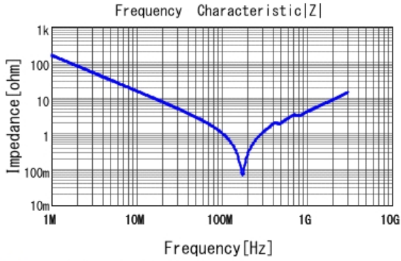
■ GCM31A7U2J102JX01 |Z| DCOV, 25degC
