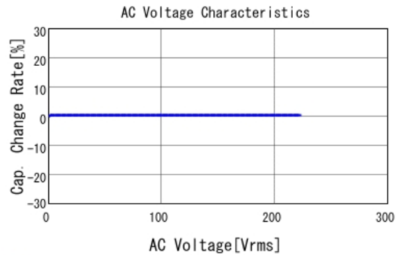
■ GCM55D7U2J473JX01 C-AC Voltage capchange, DC0V, 25.0d
