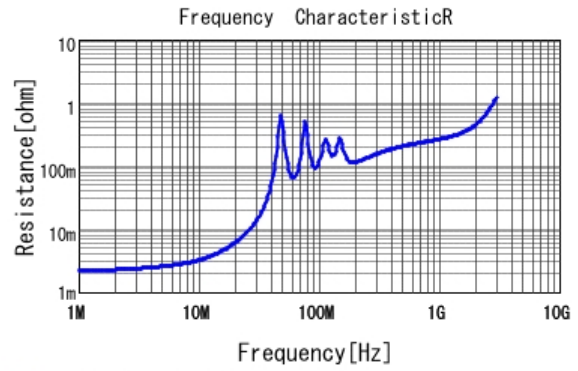
■ GCM55D7U2J473JX01 R DC0V, 25degC
