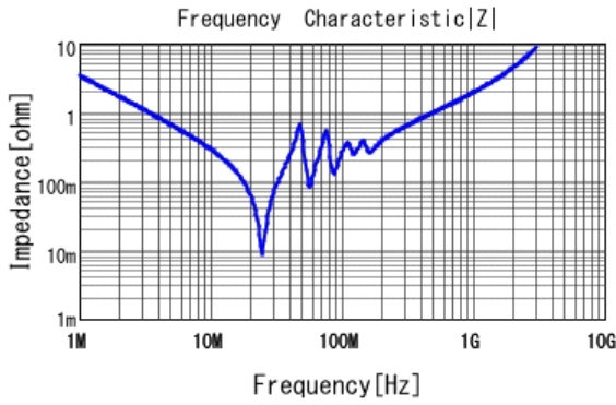
■ GCM55D7U2J473JX01 |Z| DC0V, 25degC
