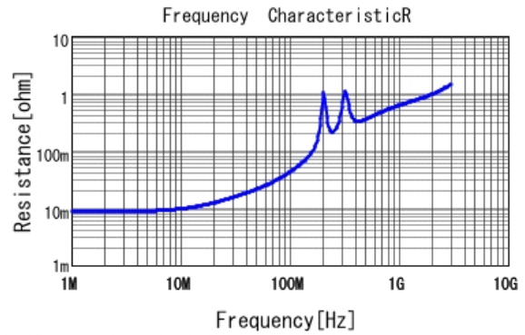
GCM31B7U2J332JX01 R DC0V, 25degC
