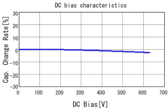
GCM31B7U2J332JX01 C-DC bias capchange, 25.0degC, AC1V
