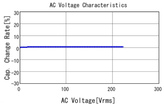
GCM31B7U2J332JX01 C-AC Voltage capchange, DC0V, 25.0d
