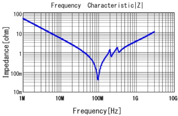
GCM31B7U2J332JX01 |Z| DC0V, 25degC
