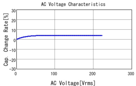
■ GCM31A7U2J221JX01 C-AC Voltage capchange, DC0V, 25.0d
