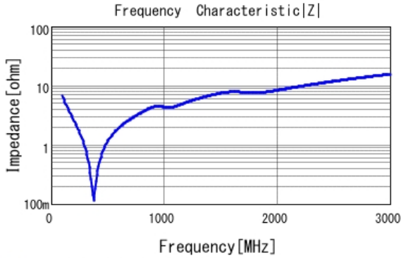
■ GCM31A7U2J221JX01 |Z| DC0V, 25degC
