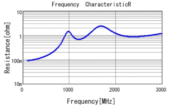
■ GCM31A7U2J221JX01 R DC0V, 25degC
