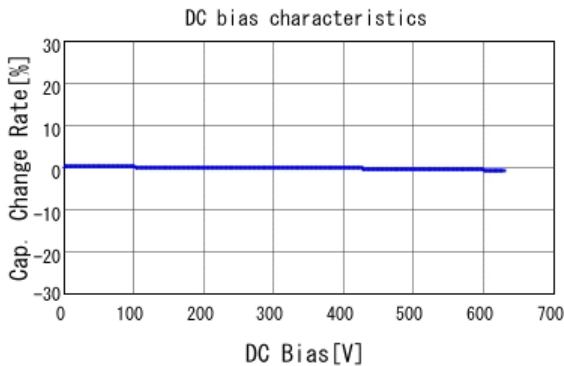
■ GCM31A7U2J221JX01 C-DC bias capchange, 25.0degC, AC1V
