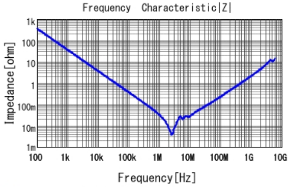
■ GCM32DC72A475KE02 |Z| DC0V, 25degC
