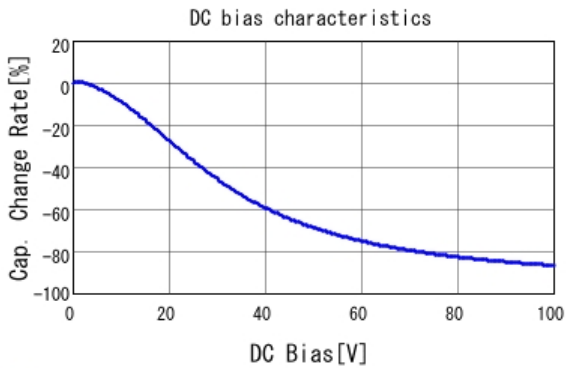
■ GCM32DC72A475KE02 C-DC bias capchange, 25.0degC, AC1.
