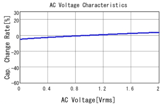
■ GCM32DC72A475KE02 C-AC Voltage capchange, DC0V, 25.0d
