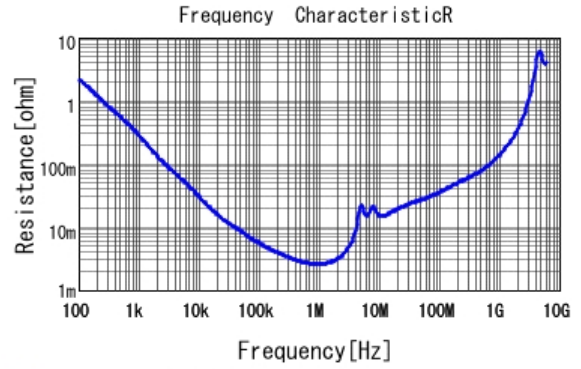
■ GCM32DC72A475KE02 R DC0V, 25degC
