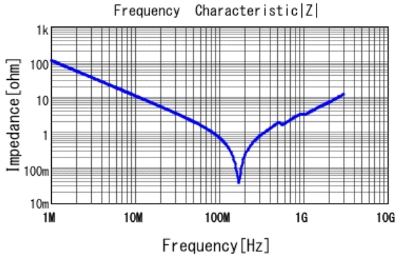
■ GCM32A7U2J152JX01 |Z| DCOV, 25degC
