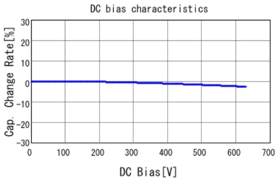
■ GCM32A7U2J152JX01 C-DC bias capchange, 25.0degC, AC1V
