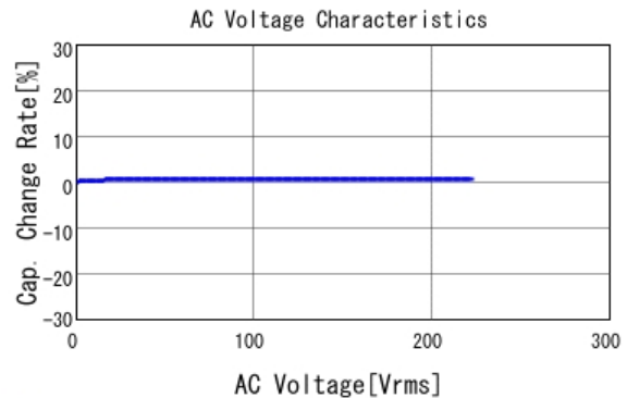
■ GCM32A7U2J152JX01 C-AC Voltage capchange, DCOV, 25.0d
