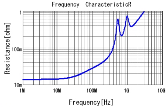
■ GCM32A7U2J152JX01 R DCOV, 25degC
