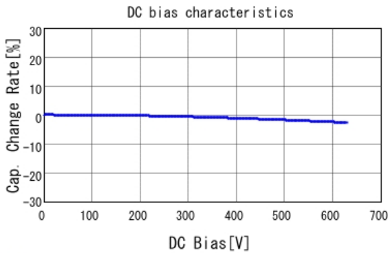
■ GCM32D7U2J103JX01 C-DC bias capchange, 25.0degC, AC1V
