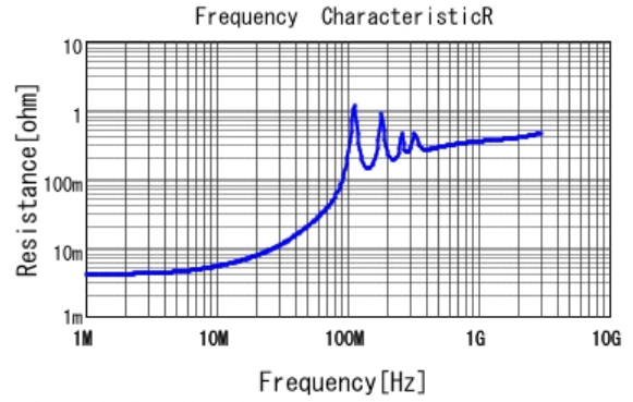
■ GCM32D7U2J103JX01 R DC0V, 25degC
