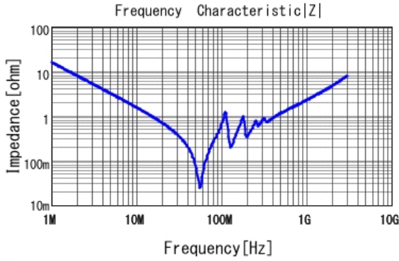
■ GCM32D7U2J103JX01 |Z| DC0V, 25degC
