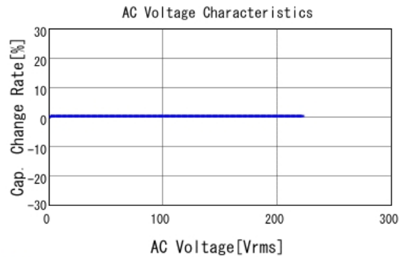
■ GCM32D7U2J103JX01 C-AC Voltage capchange, DC0V, 25.0d
