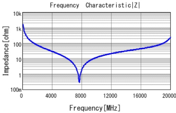
■ GCQ1555C1H1R0WB01 |Z| DC0V, 25degC
