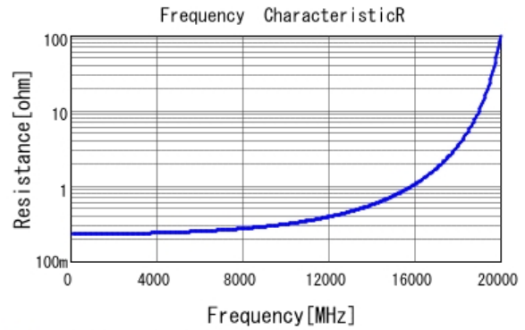
■ GCQ1555C1H1R0WB01 R DC0V, 25degC
