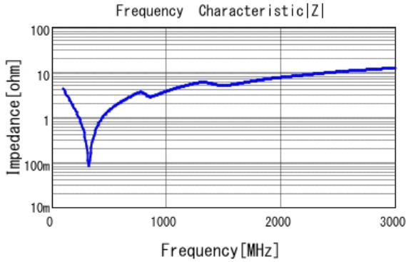
■ GCM31A7U2J331JX01 |Z| DC0V, 25degC
