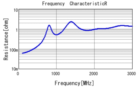
■ GCM31A7U2J331JX01 R DC0V, 25degC
