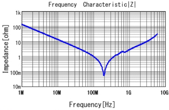
■ GCM1885C1H122JA16 |Z| DCOV, 25degC
