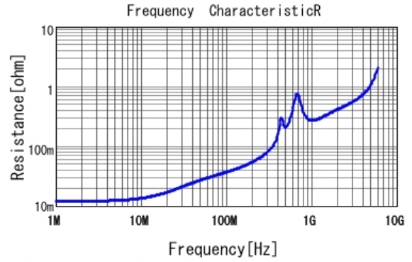
■ GCM1885C1H122JA16 R DCOV, 25degC
