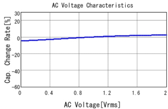
■ GCM31CC71H475KA03 C-AC Voltage capchange, DC0V, 25.0d
