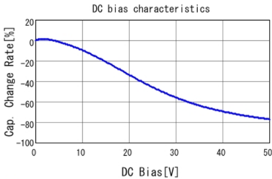
■ GCM31CC71H475KA03 C-DC bias capchange, 25.0degC, AC1.
