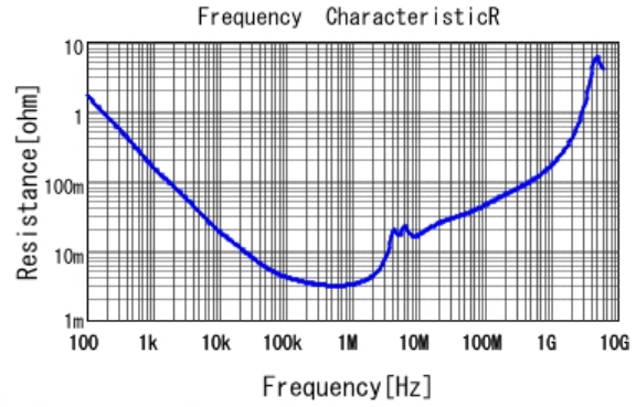
■ GCM31CC71H475KA03 R DC0V, 25degC
