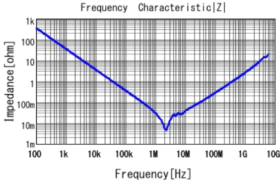
■ GCM31CC71H475KA03 |Z| DC0V, 25degC
