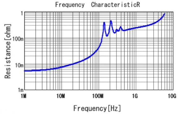
■ GCM2195C1K103JA16 R DCOV, 25degC
