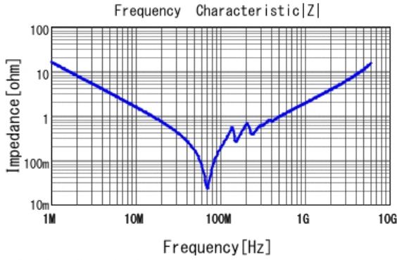
■ GCM2195C1K103JA16 |Z| DCOV, 25degC
