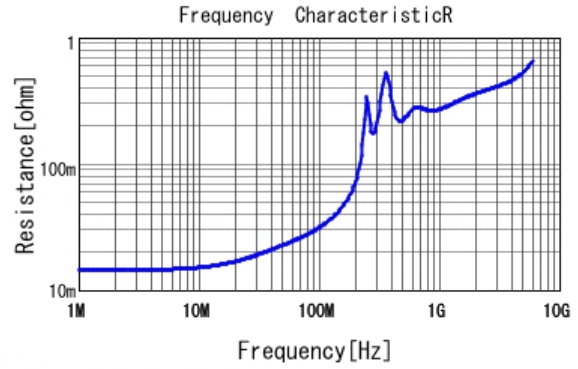
■ GCM1885C1H332JA16 R DCOV, 25degC
