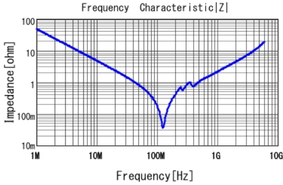
■ GCM1885C1H332JA16 |Z| DCOV, 25degC
