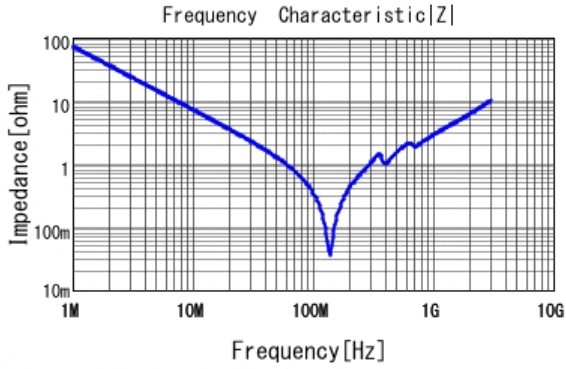
■ GCM32A7U2J222JX01 |Z| DC0V, 25degC
