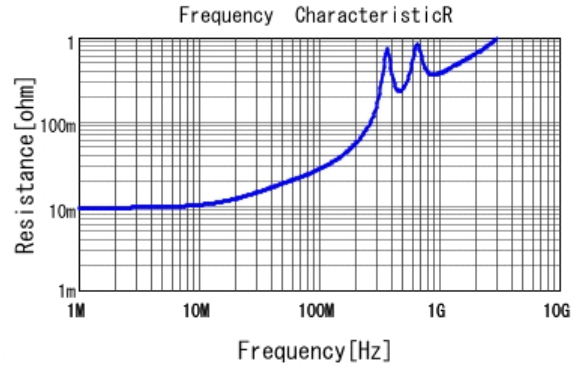
■ GCM32A7U2J222JX01 R DC0V, 25degC
