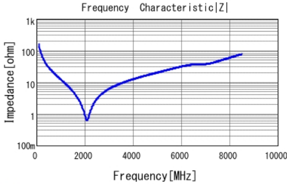
■ GCM1885C2A100JA16 |Z| DCOV, 25degC
