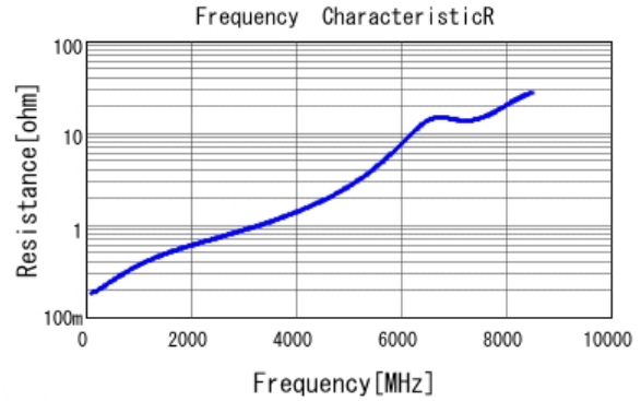
■ GCM1885C2A100JA16 R DCOV, 25degC
