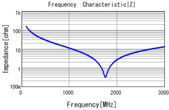
■ GCM31A7U2J100JX01 |Z| DC0V, 25degC
