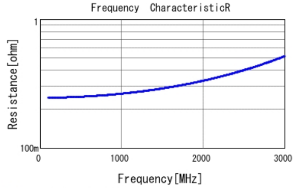
■ GCM31A7U2J100JX01 R DC0V, 25degC
