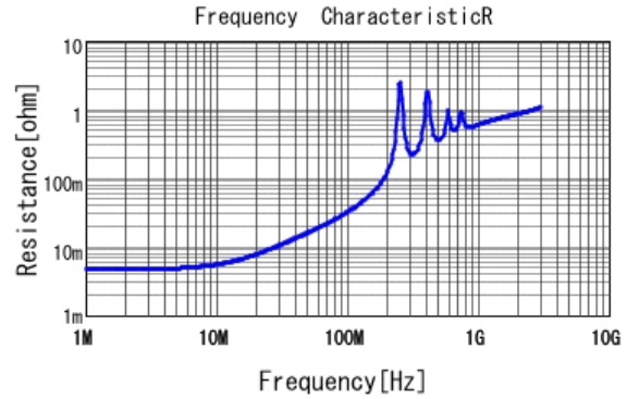
GCM32D7U3A222JX01 R DCOV, 25degC
