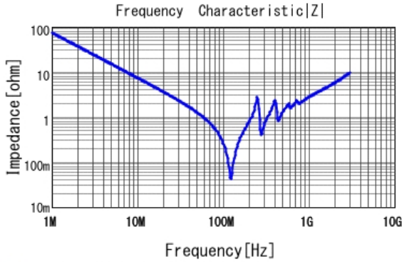
GCM32D7U3A222JX01 |Z| DCOV, 25degC
