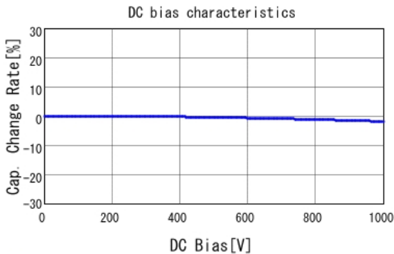
GCM32D7U3A222JX01 C-DC bias capchange, 25.0degC, AC1V
