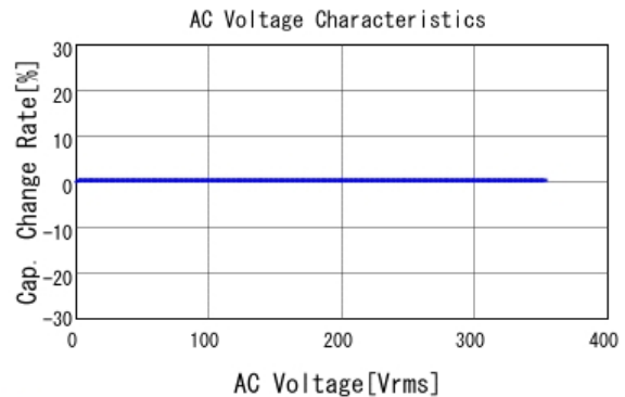
GCM32D7U3A222JX01 C-AC Voltage capchange, DCOV, 25.0d
