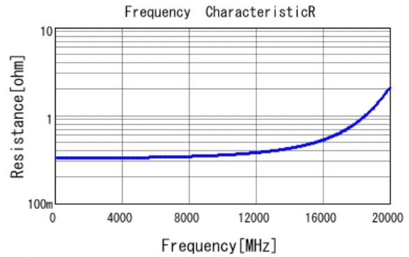
■ GCQ1555C1HR50WB01 R DCOV, 25degC
