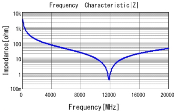
■ GCQ1555C1HR50WB01 |Z| DCOV, 25degC
