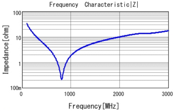
■ GCM31A7U2J470JX01 |Z| DC0V, 25degC
