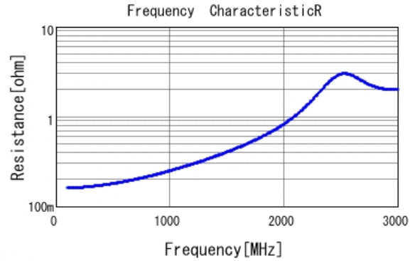
■ GCM31A7U2J470JX01 R DC0V, 25degC
