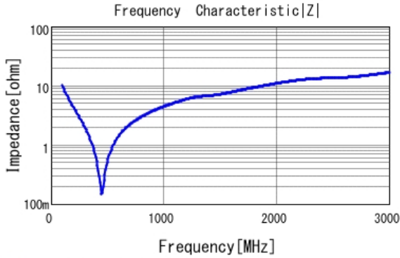
■ GCM31A7U2J151JX01 |Z| DCOV, 25degC
