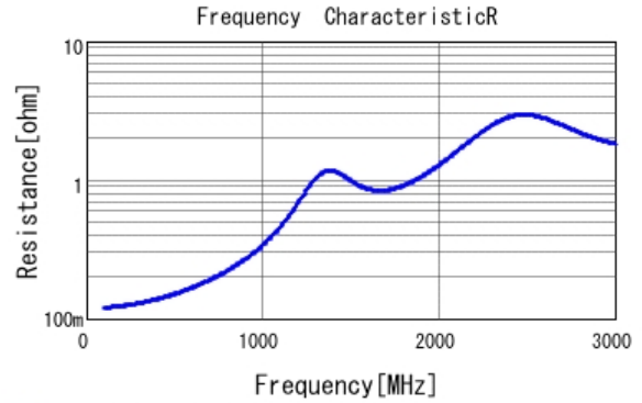
■ GCM31A7U2J151JX01 R DCOV, 25degC
