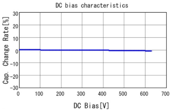
■ GCM31A7U2J151JX01 C-DC bias capchange, 25.0degC, AC1V
