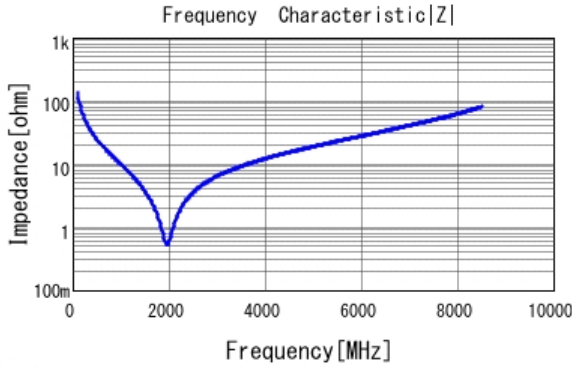
■ GCM1885C2A120JA16 |Z| DCOV, 25degC
