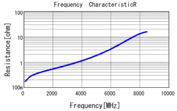
■ GCM1885C2A120JA16 R DCOV, 25degC
