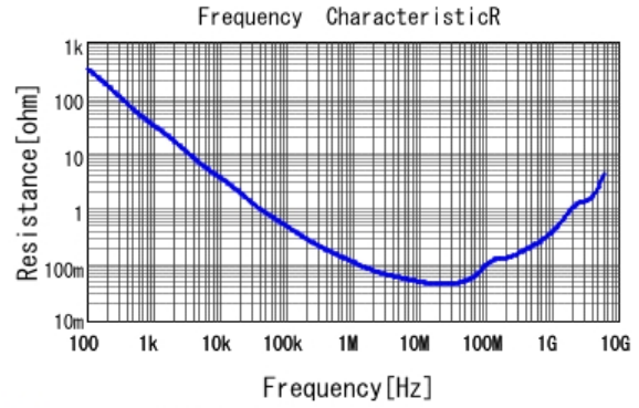
GCM188R72A223KA37 R DCOV, 25degC
