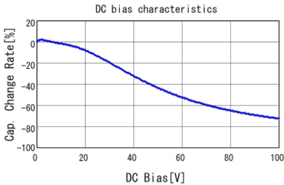
GCM188R72A223KA37 C-DC bias capchange, 25.0degC, AC1.
