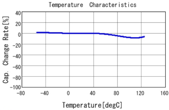
■ GCM188R72A223KA37 C-Temp. capchange, DC0.0V, AC1.0V rm
