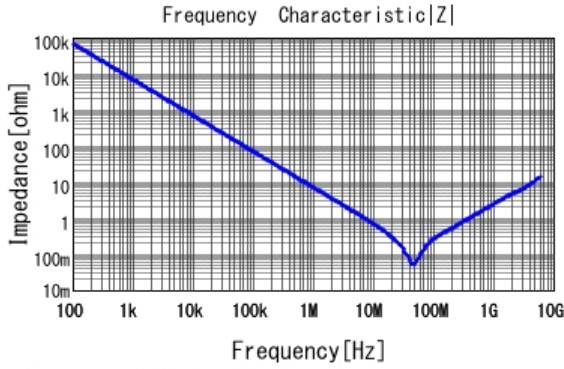
GCM188R72A223KA37 |Z| DCOV, 25degC
