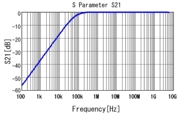
■ GCM188R72A223KA37 S21 DC0V, 25degC
