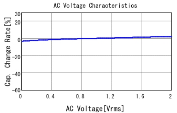
GCM188R72A223KA37 C-AC Voltage capchange, DCOV, 25.0d
