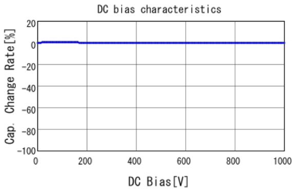
■ RCE5C3A270J2M1H03A C-DC bias capchange, 25.0degC, AC1
