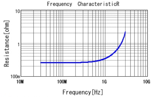
■ RCE5C3A220J2M1H03A R DCOV, 25degC
