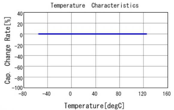
■ RCE5C3A220J2M1H03A C-Temp. capchange, DCOV, AC1Vrms
