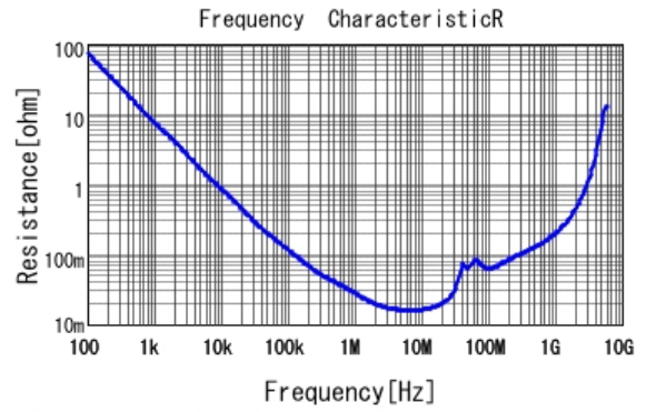
■ GCM21BR72A104KA37 R DC0V, 25degC
