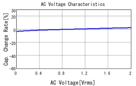
■ GCM21BR72A104KA37 C-AC Voltage capchange, DC0V, 25.0d
