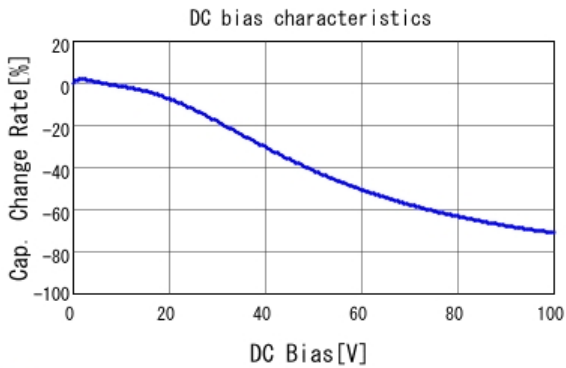
■ GCM21BR72A104KA37 C-DC bias capchange, 25.0degC, AC1.
