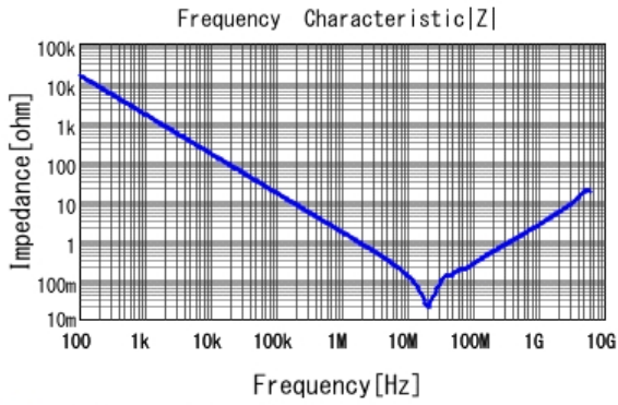
■ GCM21BR72A104KA37 |Z| DC0V, 25degC
