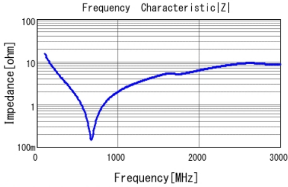
■ GRM21A5C2J101JWA1 |Z| DCOV, 25degC
