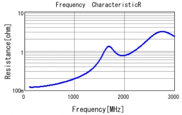
■ GRM21A5C2J101JWA1 R DCOV, 25degC
