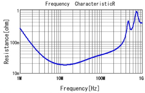
■ GRM21A5C2E122JWA1 R DC0V, 25degC
