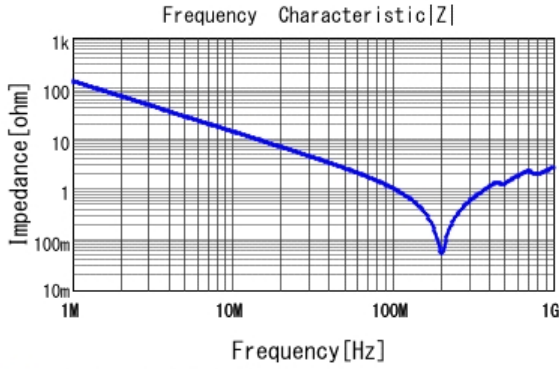
■ GRM21A5C2E122JWA1 |Z| DC0V, 25degC
