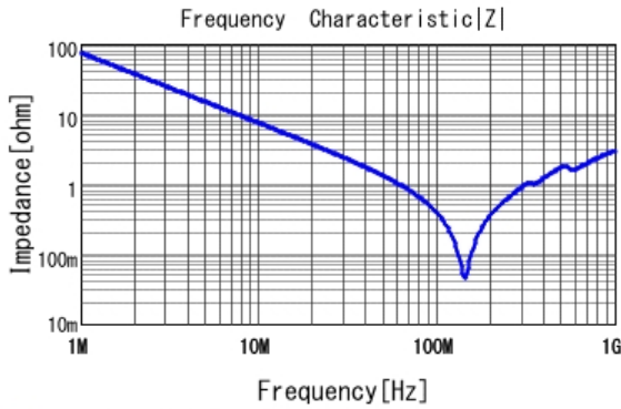
■ GRM21A5C2E222JWA1 |Z| DC0V, 25degC
