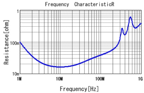
■ GRM21A5C2E222JWA1 R DC0V, 25degC
