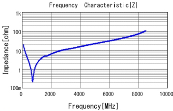
■ GCM1885C2A820JA16 |Z| DCOV, 25degC
