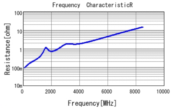
■ GCM1885C2A820JA16 R DCOV, 25degC
