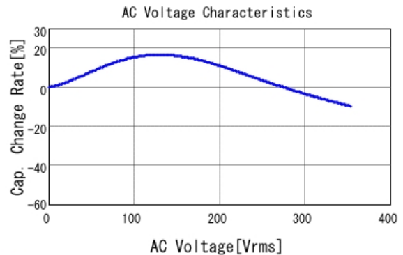
■ GCJ31BR73A472KXJ1 C-AC Voltage capchange, DC0V, 25.0d
