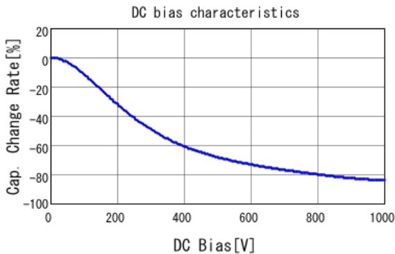
■ GCJ31BR73A472KXJ1 C-DC bias capchange, 25.0degC, AC1V
