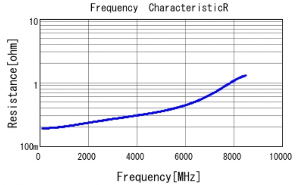
■ GRM0225C1H110GA03 R DCOV, 25degC
