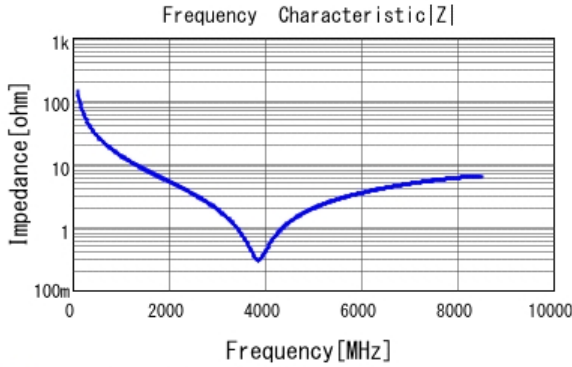
■ GRM0225C1H110GA03 |Z| DCOV, 25degC
