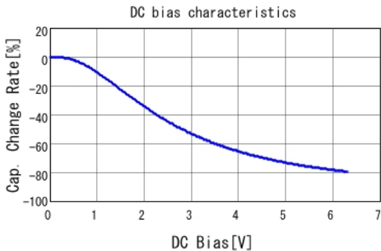
■ GRM155D80J225ME95 C-DC bias capchange, 25.0degC, ACO.
