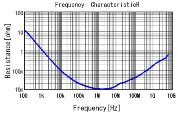
■ GRM155D80J225ME95 R DCOV, 25degC
