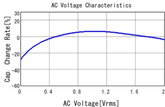
■ GRM155D80J225ME95 C-AC Voltage capchange, DCOV, 25.0d
