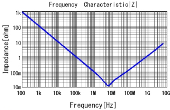
■ GRM155D80J225ME95 |Z| DCOV, 25degC
