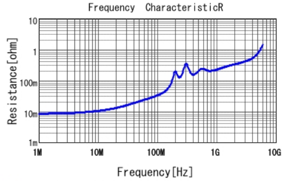
■ GRM1885C1H562JA01 R DCOV, 25degC
