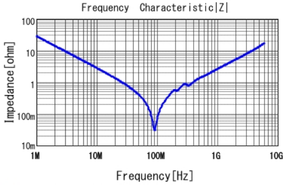
■ GRM1885C1H562JA01 |Z| DCOV, 25degC
