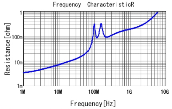
■ GRM21B5C2A183JA01 R DCOV, 25degC
