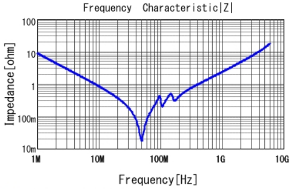
■ GRM21B5C2A183JA01 |Z| DCOV, 25degC
