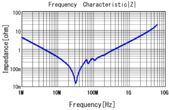
■ GRM21B7U1H393JA01 |Z| DCOV, 25degC
