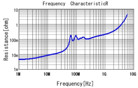
■ GRM21B7U1H393JA01 R DCOV, 25degC
