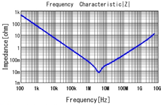
■ GRM185C81A475KE11 |Z| DCOV, 25degC
