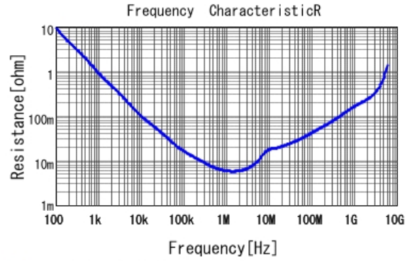
■ GRM185C81A475KE11 R DCOV, 25degC
