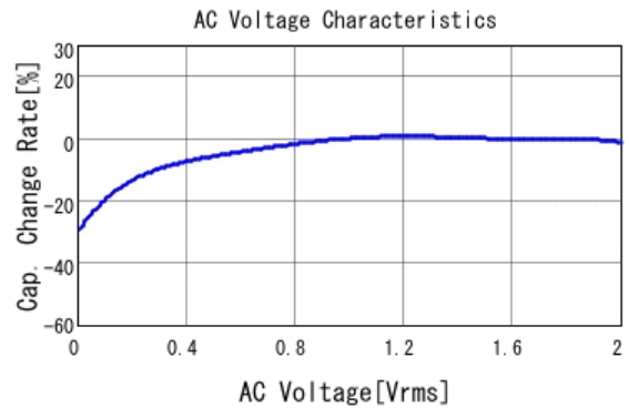
■ GRM185C81A475KE11 C-AC Voltage capchange, DCOV, 25.0d
