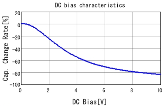
■ GRM185C81A475KE11 C-DC bias capchange, 25.0degC, AC1V
