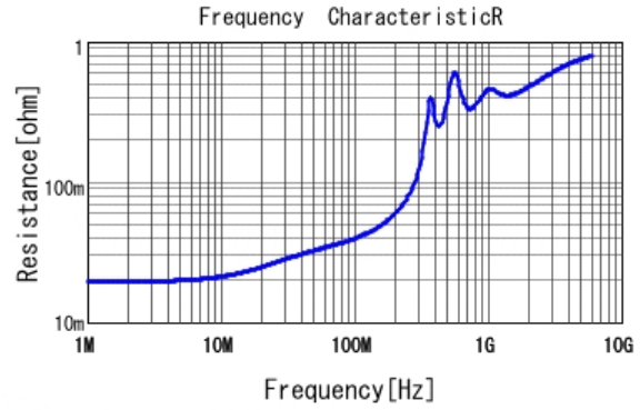
■ GRM1885C2A152JA01 R DCOV, 25degC
