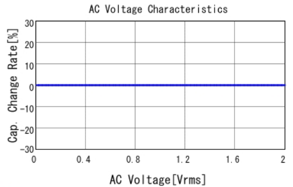
■ GRM1885C2A152JA01 C-AC Voltage capchange, DCOV, 25.0d
