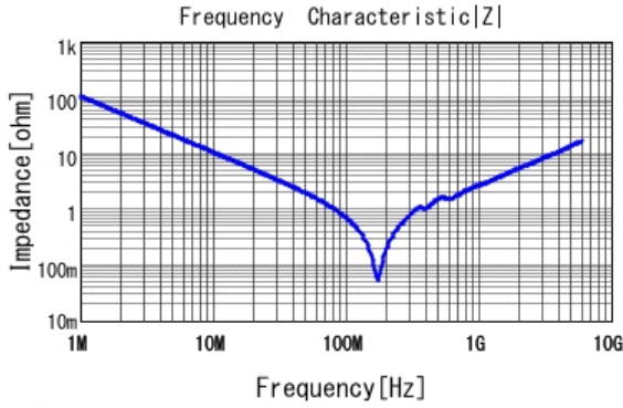
■ GRM1885C2A152JA01 |Z| DCOV, 25degC
