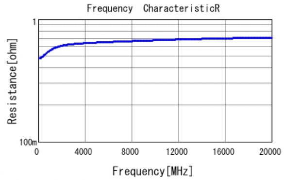
■ GRM0225C1H1R0CA03 R DCOV, 25degC
