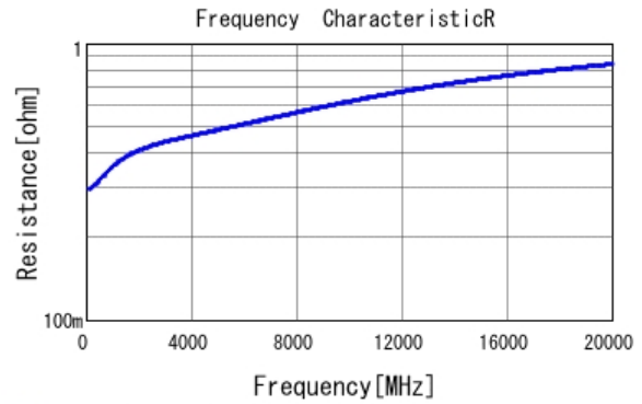
■ GRM0225C1H1R8CA03 R DCOV, 25degC
