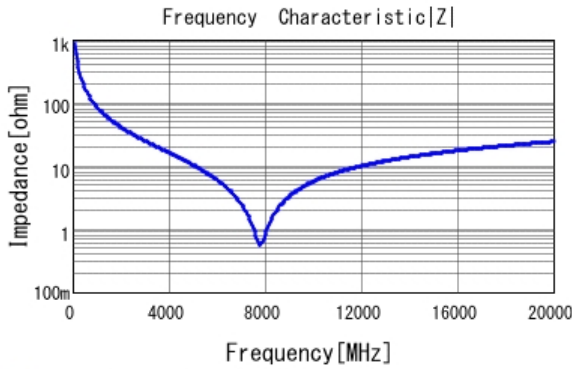
■ GRM0225C1H1R8CA03 |Z| DCOV, 25degC
