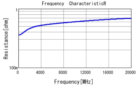
■ GRM0225C1H1R5WA03 R DCOV, 25degC
