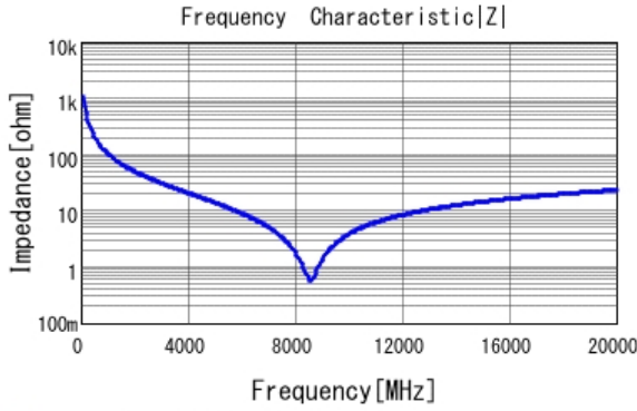
■ GRM0225C1H1R5WA03 |Z| DCOV, 25degC
