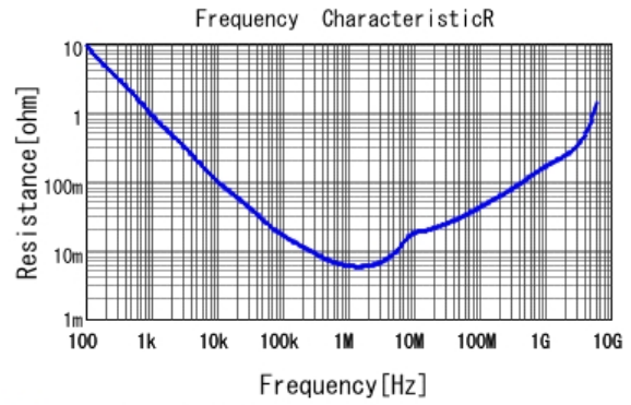
■ GRM185D70J475ME11 R DCOV, 25degC
