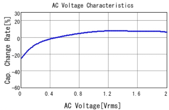
■ GRM185D70J475ME11 C-AC Voltage capchange, DCOV, 25.0d
