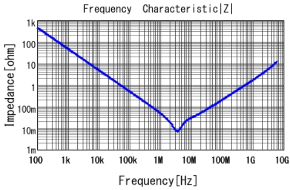
■ GRM185D70J475ME11 |Z| DCOV, 25degC
