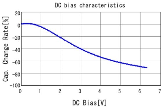
■ GRM185D70J475ME11 C-DC bias capchange, 25.0degC, ACO.
