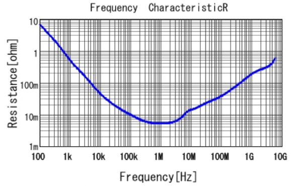
■ GRM155R60J475ME47 R DCOV, 25degC
