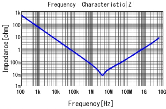
■ GRM155R60J475ME47 |Z| DCOV, 25degC
