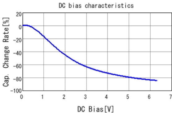
■ GRM155R60J475ME47 C-DC bias capchange, 25.0degC, AC0.
